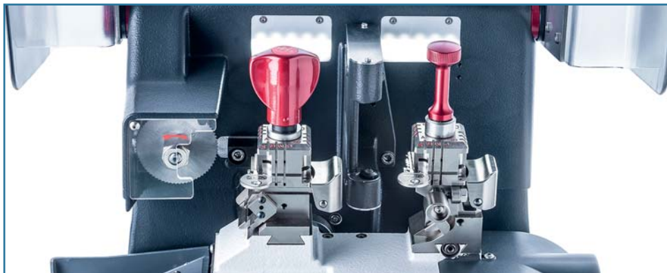
Key cutting station with AlCrN coated cutter
