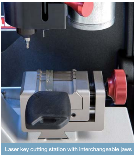
Flat key cutting station with fast-rotating clamp
